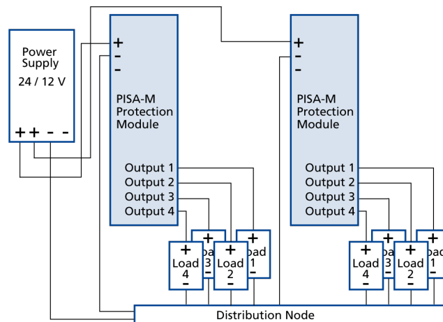
Fig. 3-2: Wiring scheme for multiple PISA-M modules connected to one power supply with nominal output current > 20 A
