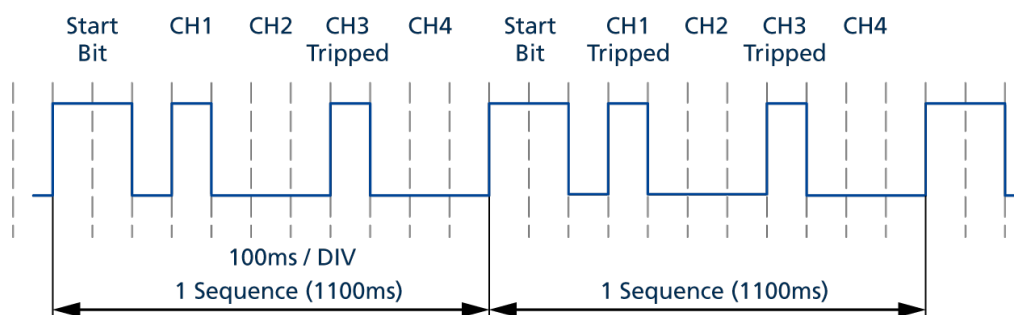
Fig. 16-1: Digital Coded Sequence (unidirectional) – PISA-M to PLC
